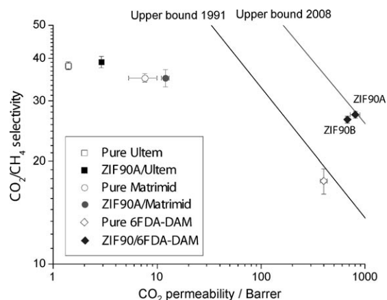
Figure 3. Gas-permeation properties of mixed-matrix membranes containing 15 wt% of ZIF-90 crystals measured with pure gases. Measurements were performed at 35^\circ\text{C} and 4.5 atm upstream pressure for Ultem and Matrimid membranes, and at 25^\circ\text{C} and 2 atm upstream pressure for 6FDA-DAM membranes. The data for pure Ultem and Matrimid are averaged values from the literature. [13b, 24] The upper bounds for polymer membrane performance as defined in 1991 and 2008 are shown.
