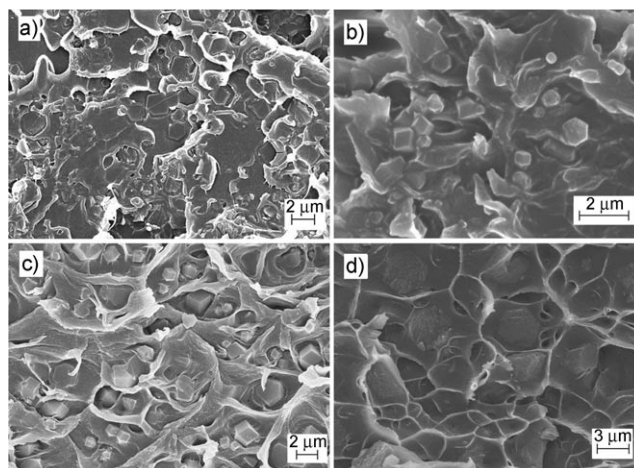
Figure 2. SEM images of cross-sections of mixed-matrix membranes containing ZIF-90 crystals; a) ZIF-90A/Ultem, b) ZIF-90A/Matrimid, c) ZIF-90A/6FDA-DAM, and d) ZIF-90B/6FDA-DAM.
