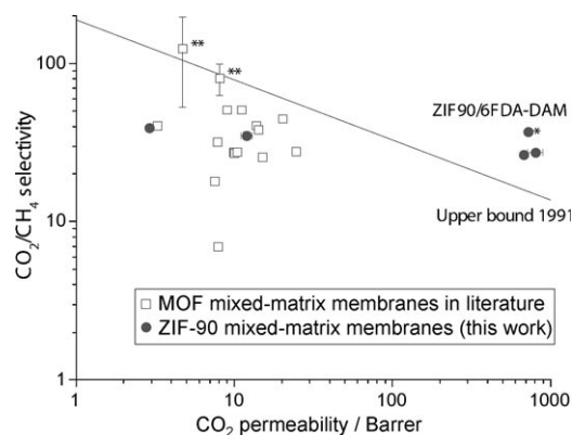
Figure 4. CO 2 /CH 4 separation performance of the present ZIF-90 mixed-matrix membranes, compared with the compiled data on MOF-containing mixed-matrix membranes. [15–18,25] Data marked with * is based upon our mixed-gas permeation measurements. Data from previous work marked with ** carries a large error bar owing to inaccuracy in measuring low permeabilities. [25] The upper bound for polymer performance as defined in 1991 is shown.
