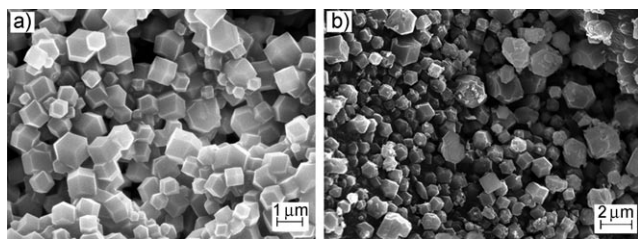
Figure 1. SEM images of submicrometer-sized ZIF-90 particles; a) ZIF-90A synthesized using methanol as a nonsolvent; b) ZIF-90B synthesized using deionized water as a nonsolvent.
